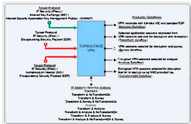
(TS//SI//REL) TU VPN Products
