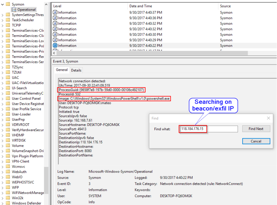
Figure 6 – Searching Sysmon for the exfil IP
